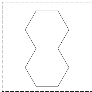
honey comb 4 \frac{27}{32}'' \times 8 \frac{13}{32}'' \times \frac{3}{8}'' coverage: 0.21 sqft/pcs
