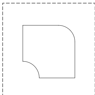
ruffle 6 \frac{15}{32}'' \times 6 \frac{15}{32}'' \times \frac{3}{8}'' coverage: 0.26 sqft/pcs
