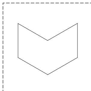
ravel 3 \frac{17}{32}'' \times 6 \frac{1}{8}'' \times \frac{3}{8}'' coverage: 0.15 sqft/pcs
